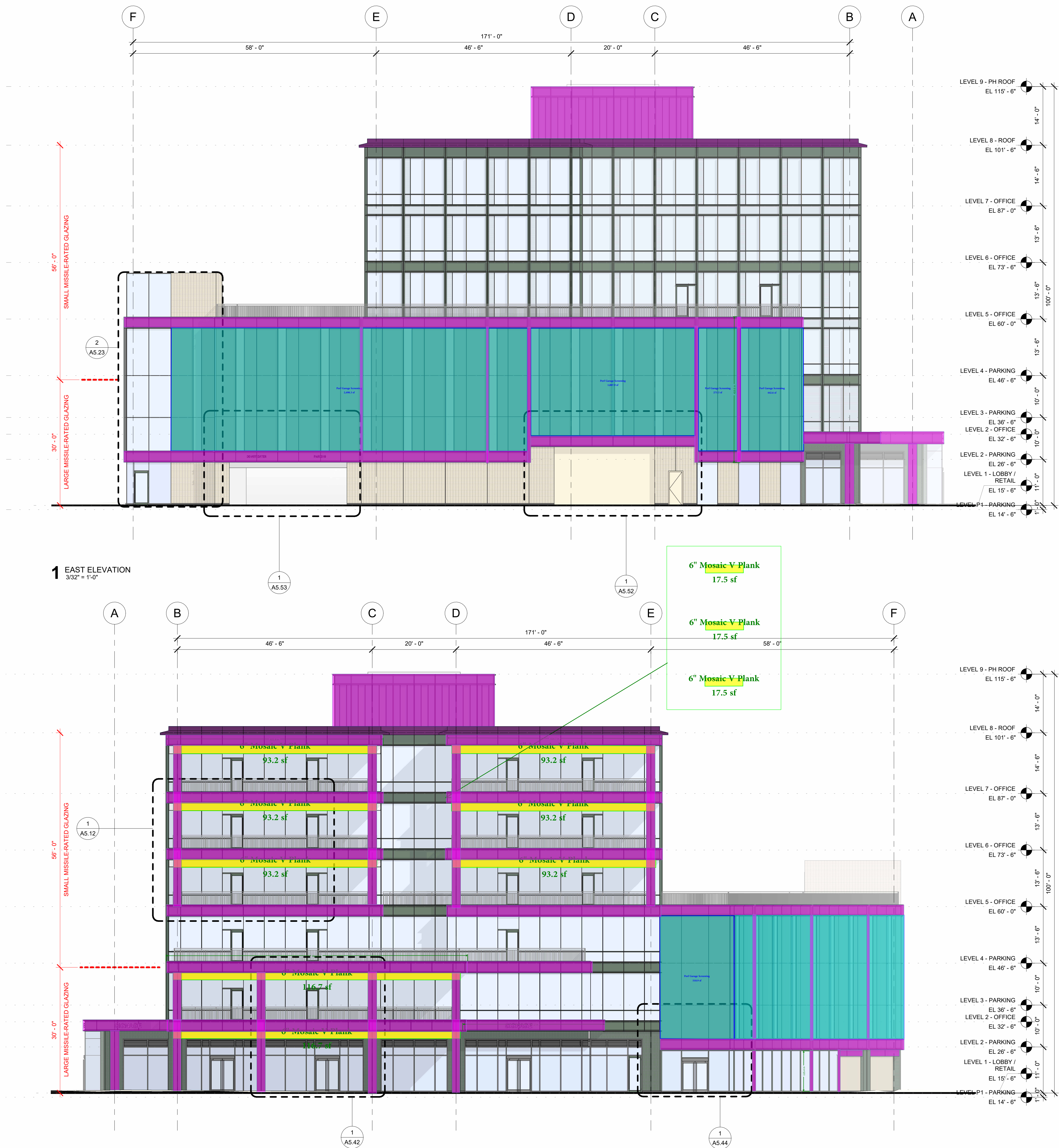
2 WEST ELEVATION 3/32" = 1'-0"
