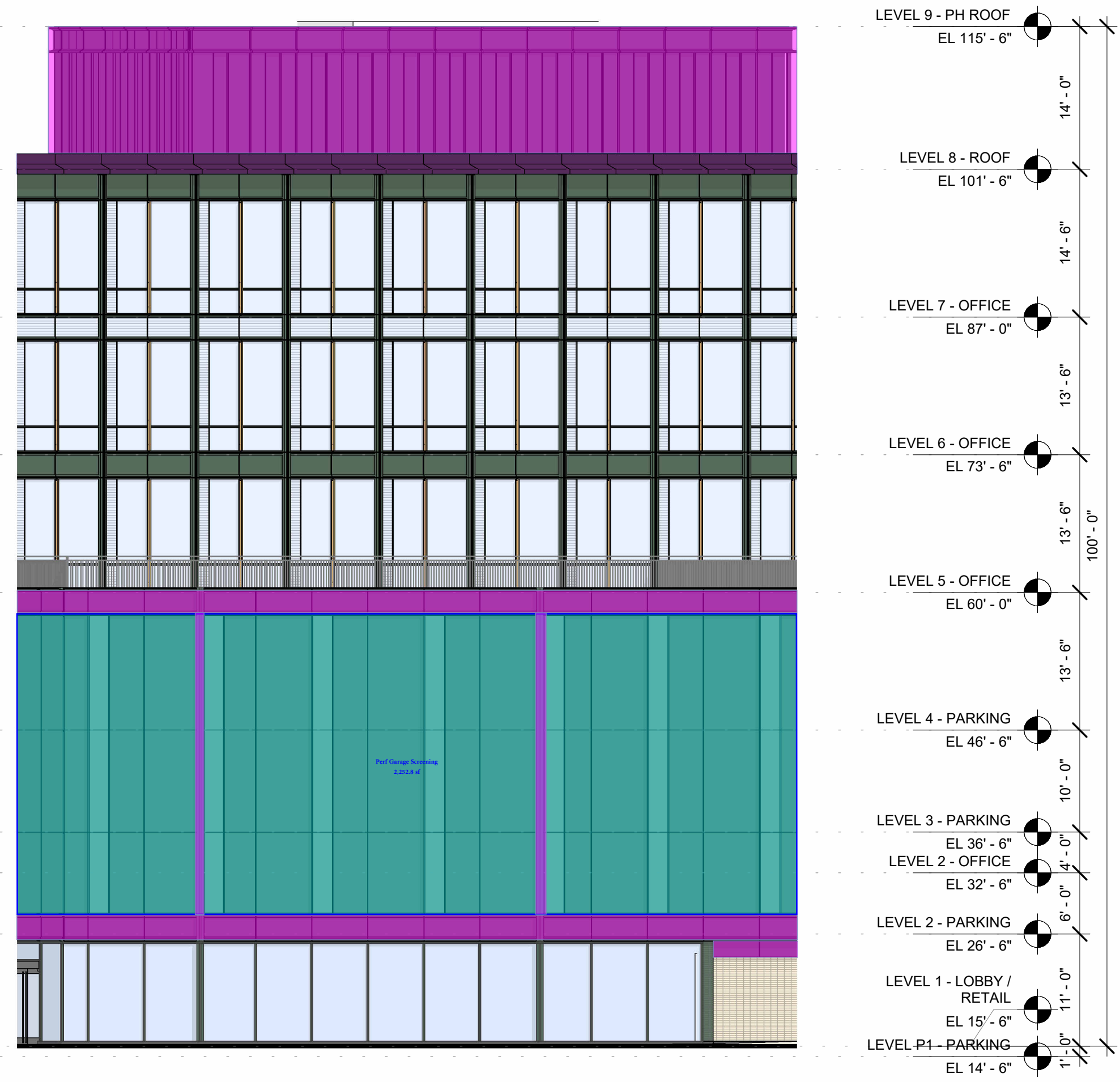
3 SOUTHWEST ELEVATION 3/32" = 1'-0"
